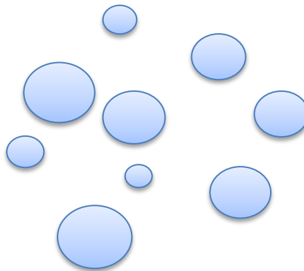
polydispers
