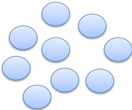
monodispers
