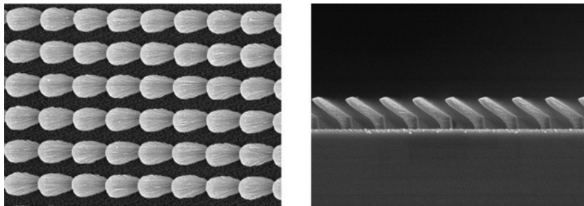
Pre-patterned substrates
