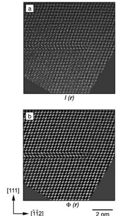
Figure 10. Multiple stacking fault in GaAs laterally bound by a partial dislocation. (a) Optimum defocus image, I(r) . (b) Reconstructed exit plane phase, \Phi(r) , showing enhanced contrast and lower noise levels. (Reproduced with
