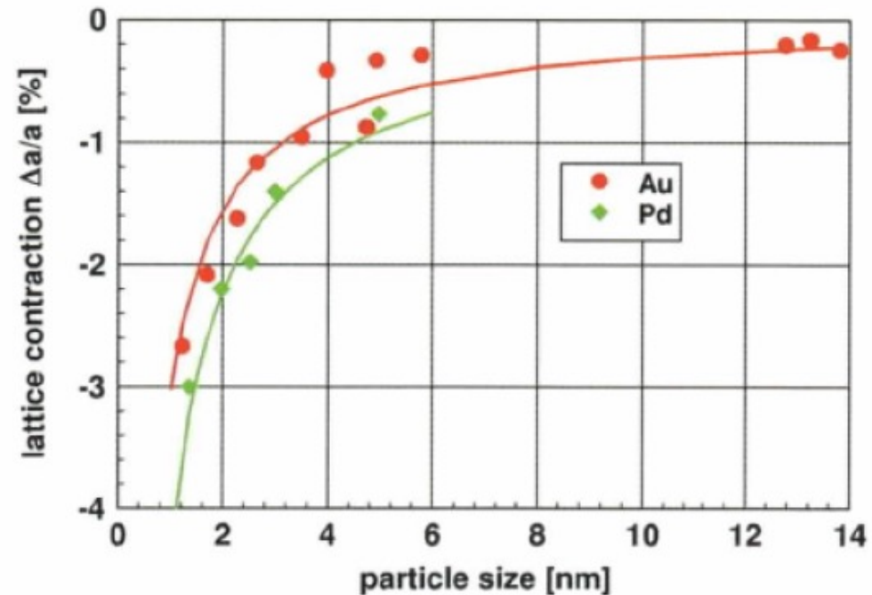
Figure 2.15 Experimental values for the lattice constant of gold [11] and palladium [12] nanoparticles. Due to hydrostatic pressure originating from surface tension, decreasing lattice parameters are observed with decreasing particle size.
