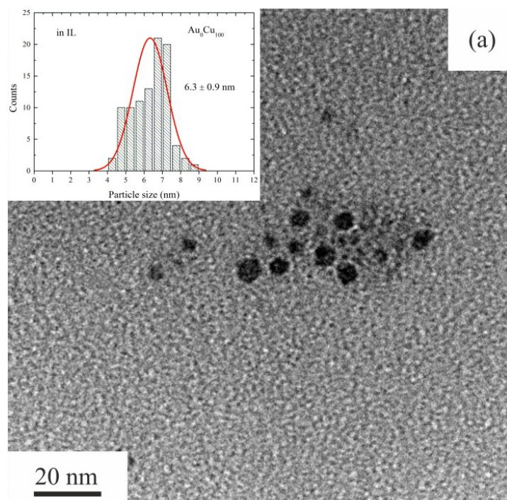
(a) TEM of Cu NPs in [C 1 C 4 im][Tf 2 N] (b) HRTEM of a single Cu NP in IL
