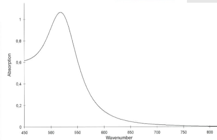
Figure 2.3 UV-visible spectrum of 18-nm gold particles.
