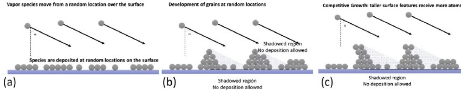
Fig. 4.1. First stages of growth during the OAD of thin films. (a) Individual vapor species arrive at random locations on the surface with a given tilt angle. (b) Deposited particles accumulate within certain regions in the form of grains of material that then cast shadows over other surface zones where vapor species cannot be deposited. (c) Taller surface features are more likely to grow, initiating a competitive growth process in which the taller a feature is the larger its shadow, thus forming tilted columnar structures.
