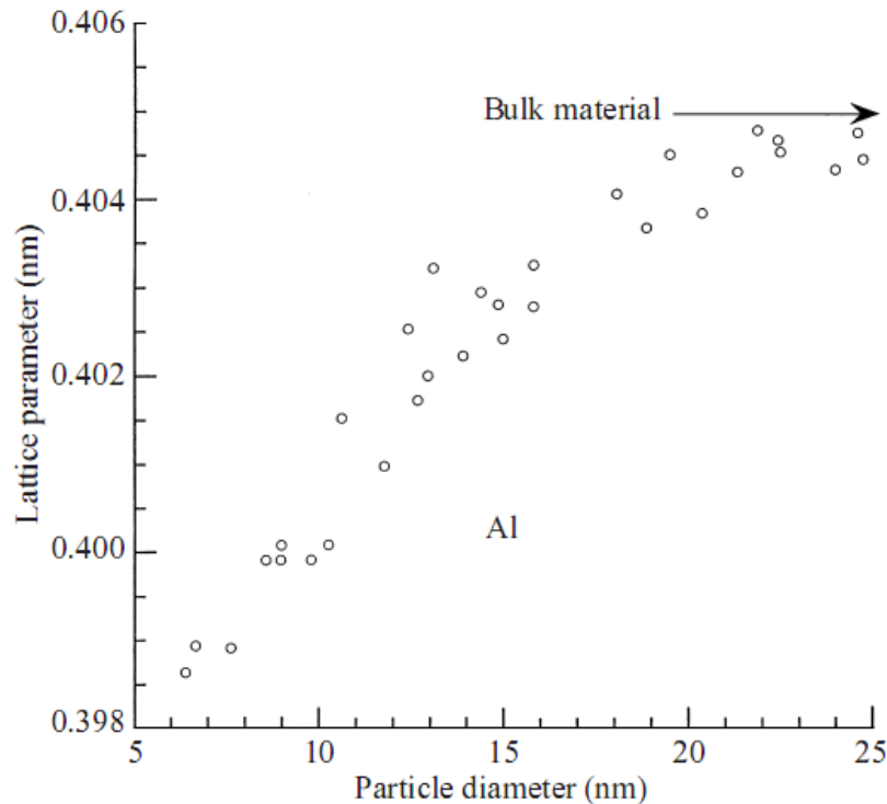
Figure 6 Reduction of the lattice constant of aluminum nanoparticles as a function of particle size (after Woltersdorf et al. 1981).
