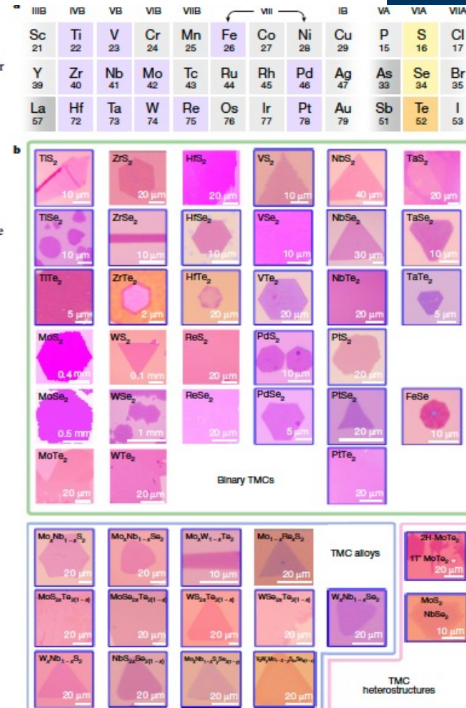
Fig. 2 | The transition metals and chalcogens used, and optical images of the resulting 47 different atomically thin TMCs and heterostructures. a, Overview of metals (highlighted in purple) and chalcogens (highlighted in yellow and orange) that can form layered sulfides, selenides and tellurides. b, Optical images of 47 TMCs synthesized using our method: binary 2D crystals containing Mo (MoS 2 , MoSe 2 , MoTe 2 ), W (WS 2 , WSe 2 , WTe 2 ), Re (ReS 2 , ReSe 2 ), Ti (TiS 2 , TiSe 2 , TiTe 2 ), Zr (ZrS 2 , ZrSe 2 , ZrTe 2 ), Hf (HfS 2 , HfSe 2 , HfTe 2 ), V (VS 2 , VSe 2 , VTe 2 ), Nb (NbS 2 , NbSe 2 , NbTe 2 ), Ta (TaS 2 , TaSe 2 , TaTe 2 ), Pt (PtS 2 , PtSe 2 , PtTe 2 ).
