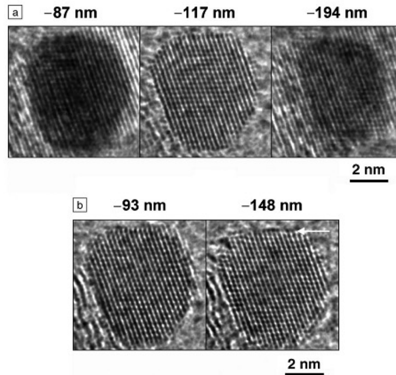
Figure 9. (a) Through-focal series of images of a nanocrystalline Pt particle supported on partially graphitized carbon with a spherical aberration of 450 \mu\text{m} . (b) Equivalent focal series of the same particle after aberration correction with a spherical aberration of -20 \mu\text{m} . In both (a) and (b), defocus values are indicated, with negative values corresponding to underfocus. In (a), extensive contrast delocalization as a function of defocus is observed, which is eliminated in (b). A partially complete surface layer is marked with an arrow in (b).
