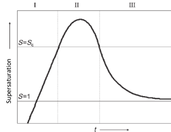
LaMer-Diagramm for changing of the supersaturation during reaction.
