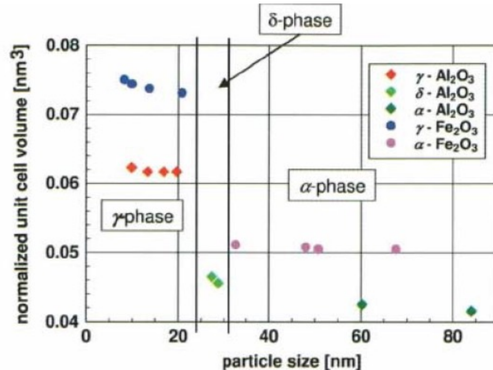
Figure 3.14 Normalized unit cell volume for different Al 2 O 3 and Fe 2 O 3 phases as a function of grain size [15]. Normalization provides a constant number of formula units per unit cell; otherwise, comparison is impossible. In the γ-phase, the unit cell volume is increased as the particle size decreases. A preference for high-temperature structures as the particle size decreases is clearly visible.
