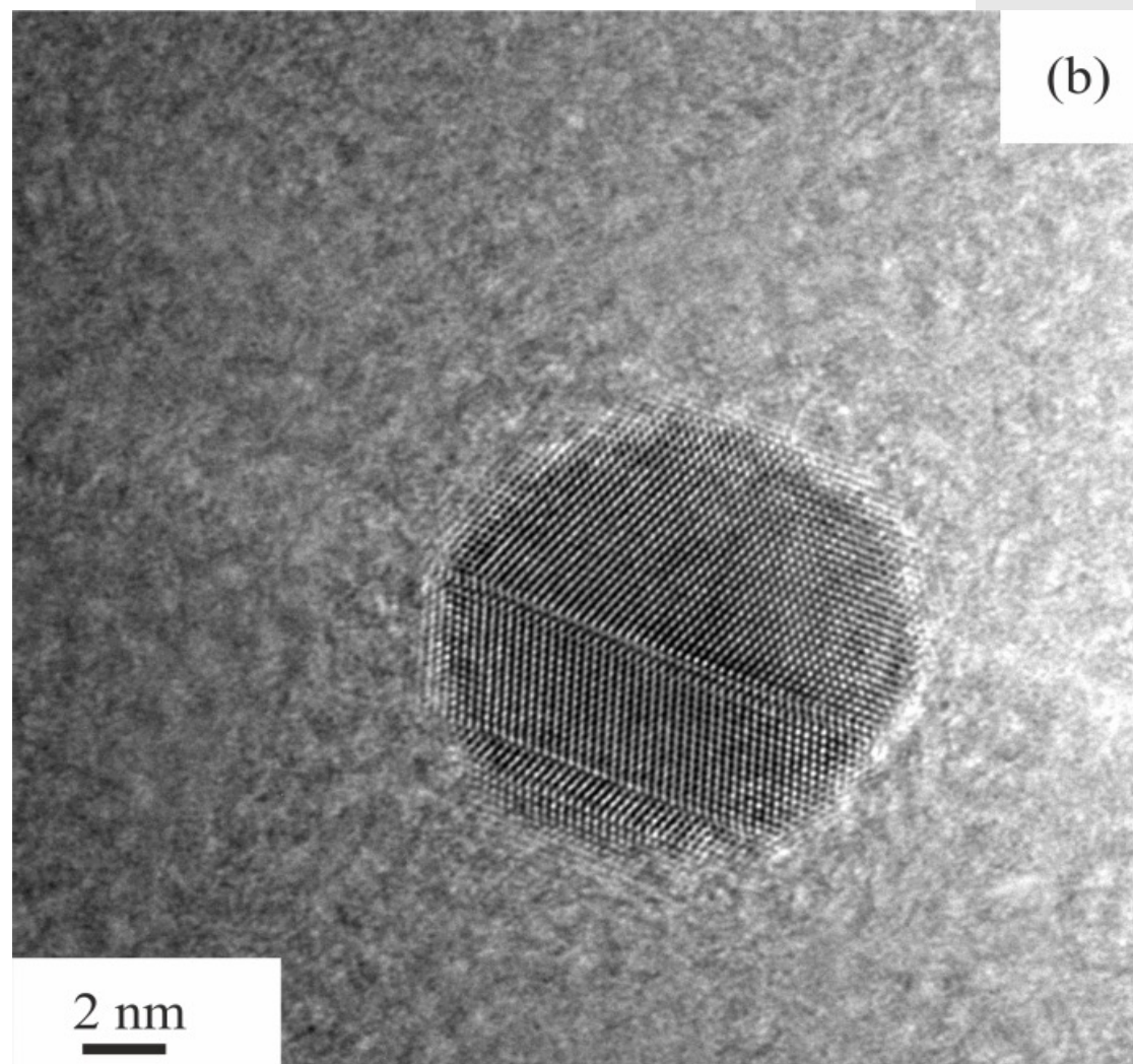
(a) TEM of Cu NPs in [C 1 C 4 im][Tf 2 N] (b) HRTEM of a single Cu NP in IL
