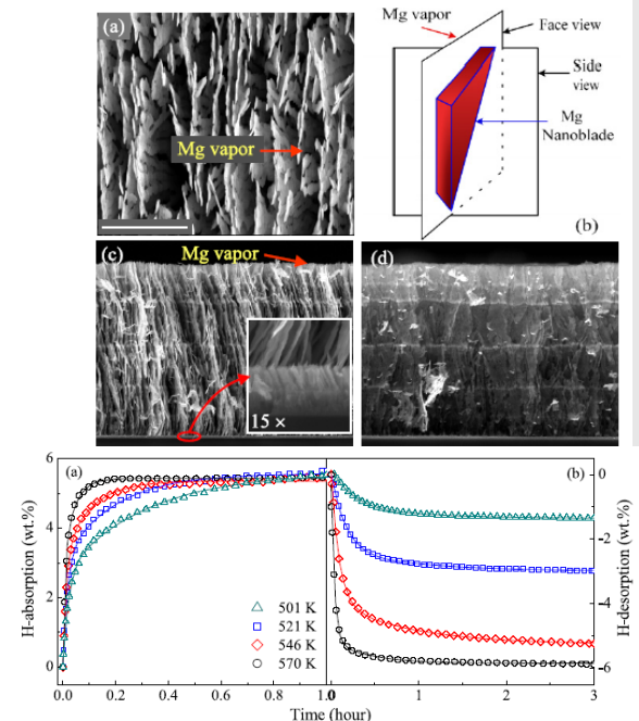
# Hydrogen storage: Mg nanoblades decorated with V
