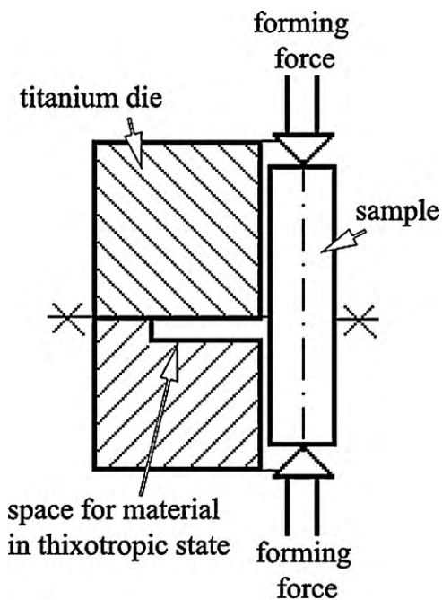
Fig. 3. Diagram of thixoforming.
