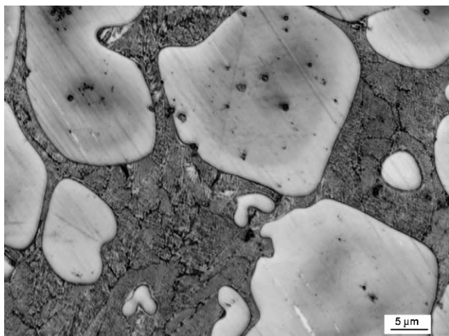
Fig. 5. Detail of carbide network area at exposure temperature of 350 °C.
