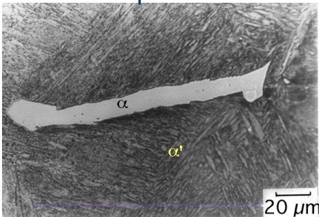
allotriomorpher Ferrit
